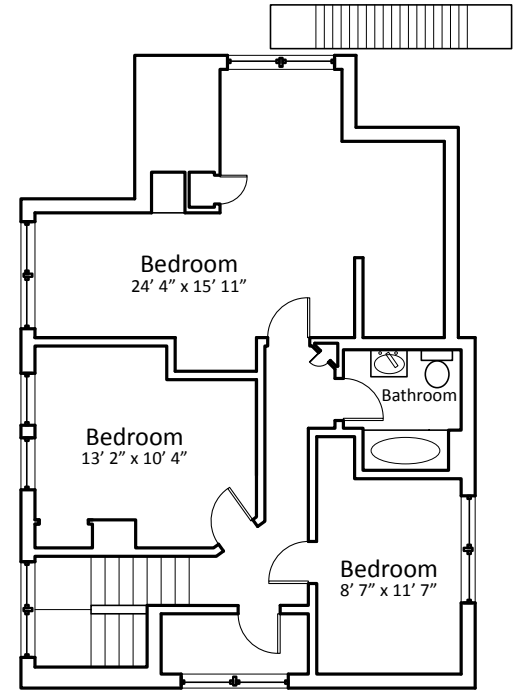
3rd Floor
